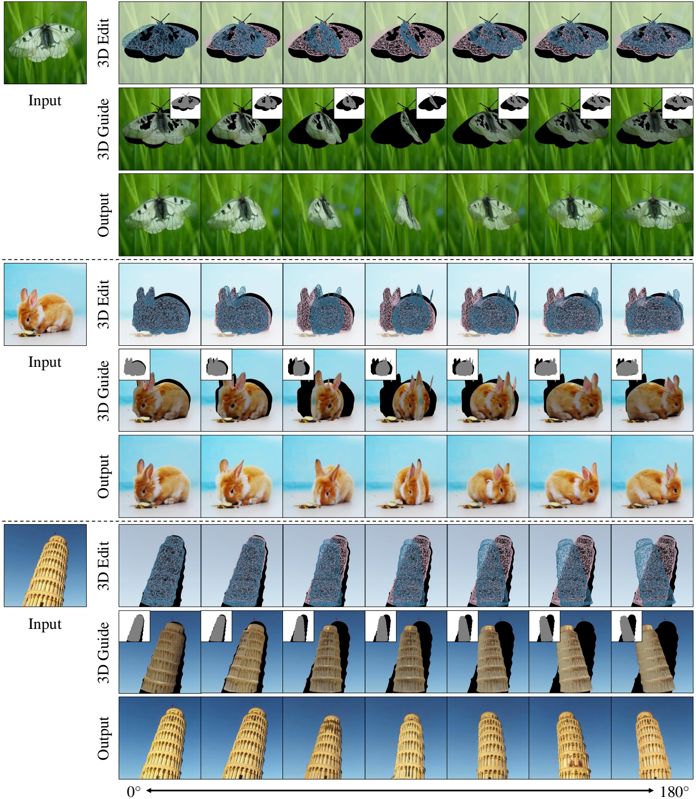
Fig. 8. 3D editing with continuous rotations. We demonstrate that the proposed method can handle extensive 3D edits on common objects. In each scenario, we progressively increase the rotation from 0 to 180 degrees along the y-axis, applying it to the reconstructed mesh to generate the 3D-transformation-based image guidance. The results show that our method can handle large out-of-plane 3D rotations during editing.
